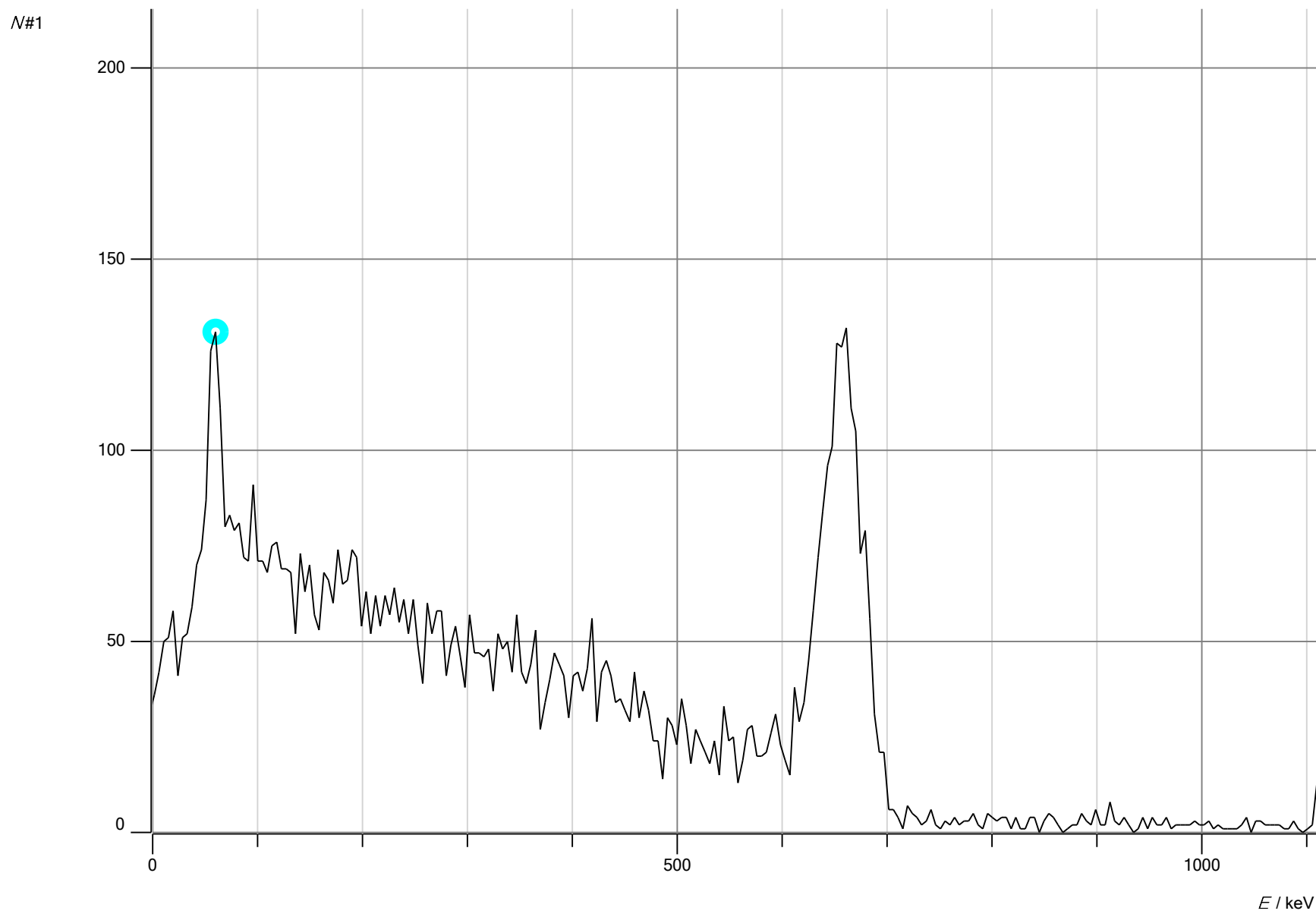
Energy Calibration - Target - Brass (Data with evaluation and fitting) - CASSY Lab 2
